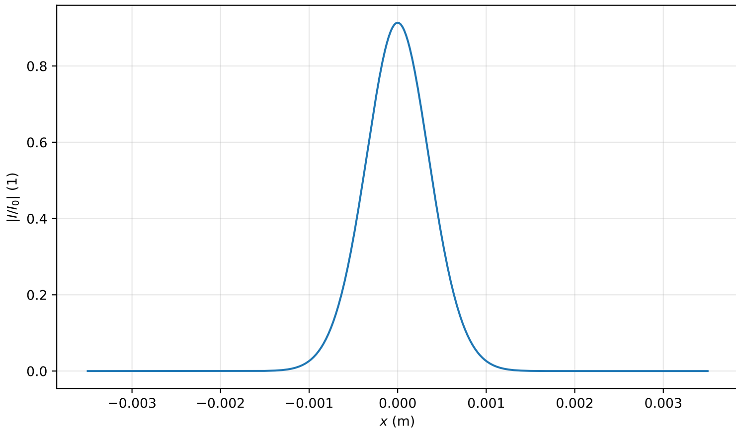
Intensity profile I(x, y = 0, z = 0.876m)/I_0 , P_{in}=0.2P_{cr} , artificial time
